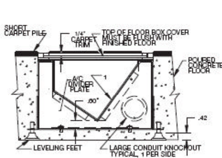
Installation Cross Section
